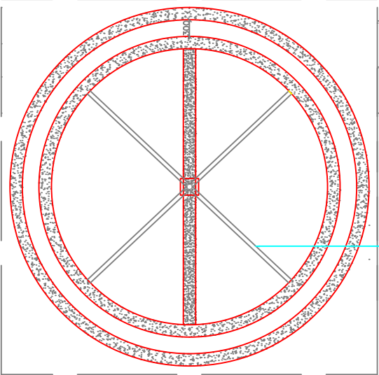
ANAEROBIC DIGESTER ( TOP VIEW ) PLAN
