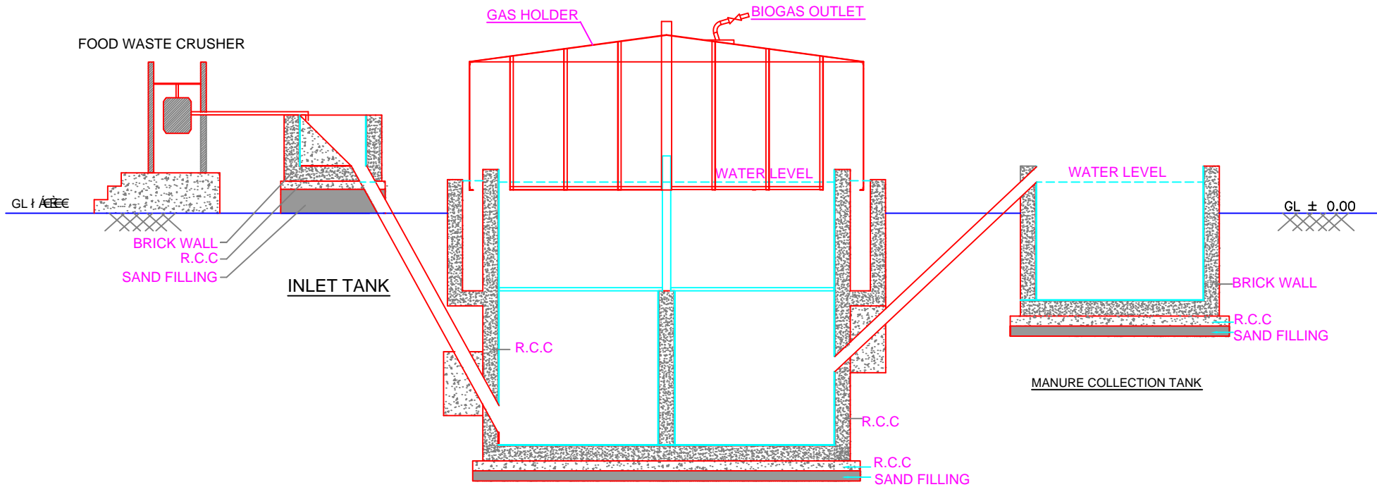
ANAEROBIC DIGESTER SECTION - AA
